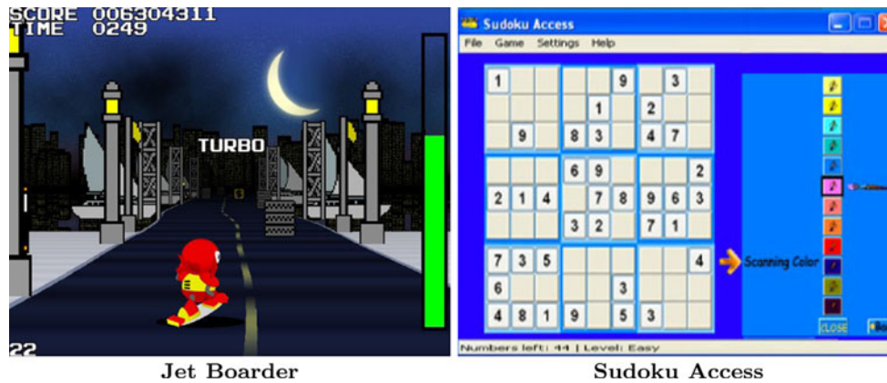
Fig. 4 One-switch games
