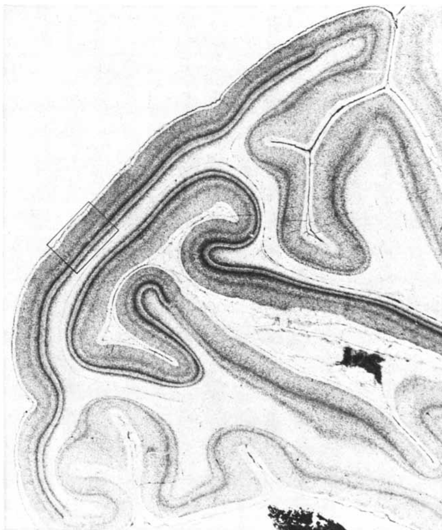
SECTION OF VISUAL CORTEX along the colored line in the illustration on the opposite page was stained by the Nissl method, which makes cell bodies but not fibers visible. The visual cortex is seen to be a continuous layered sheet of neurons about two millimeters thick. The black rectangle outlines a section like the one that is further enlarged in the illustration below.
